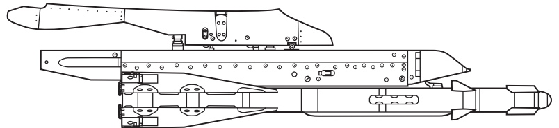
PD-62-8 pylon shown with APU-60-1 launch rail and Aphid missile (Both sold separately)
